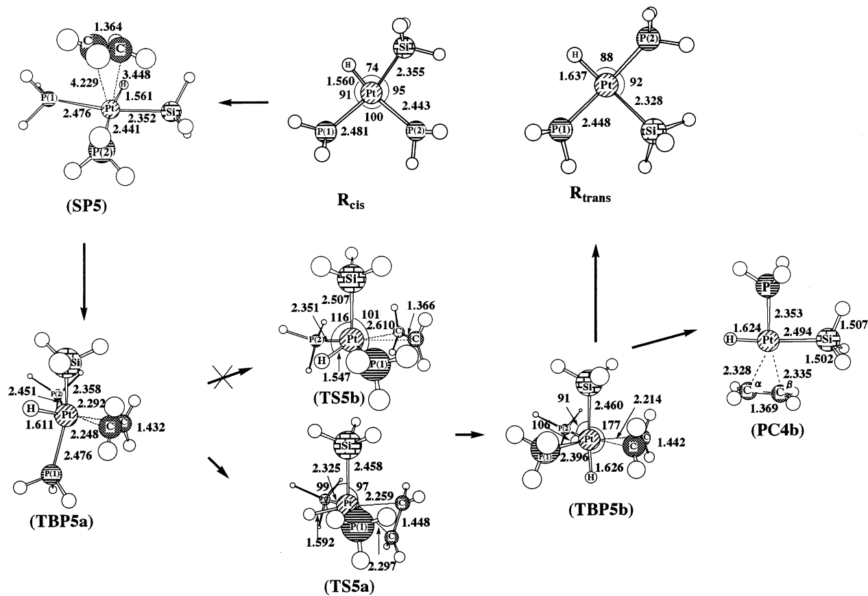
Fig. 2. Geometry changes of \text{C}_2\text{H}_4 -promoted cis - trans isomerization of \text{PtH}(\text{SiH}_3)(\text{PH}_3)_2 (bond length in Å and bond angle in degree).
