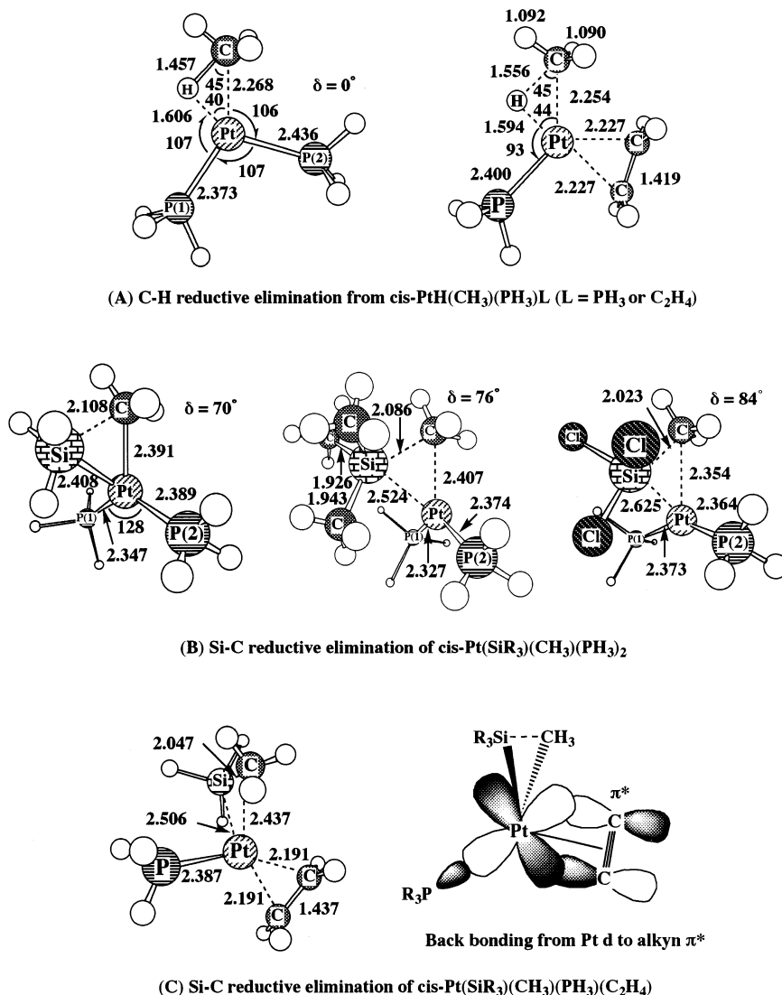
Fig. 6. Transition states of C-H and Si-C reductive elimination of \text{cis-PtH}(\text{CH}_3)(\text{PH}_3)\text{L} ( \text{L} = \text{PH}_3 or \text{C}_2\text{H}_4 ) (bond length in Å and bond angle in degree).
