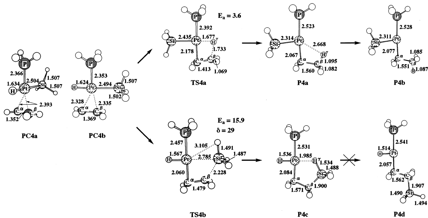
Fig. 5. Geometry changes in the ethylene insertion into Pt-H and Pt-SiH 3 bonds of trans -PtH(SiH 3 )(PH 3 )(C 2 H 4 ) (bond length in Å and bond angle in degree).
