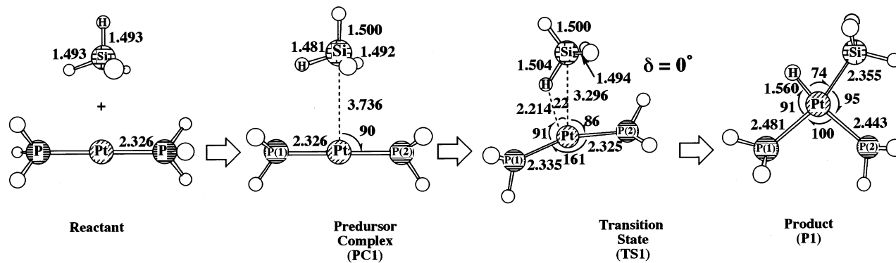
Fig. 1. Geometry changes in the Si-H oxidative addition of \text{SiH}_4 to \text{Pt(PH}_3)_2 (bond length in Å and bond angle in degree).
