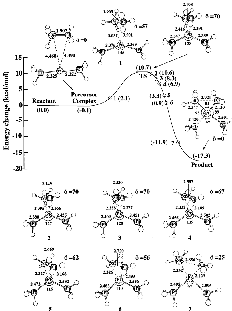
Fig. 7. Changes of total energy and geometry in the \text{SiH}_3\text{--CH}_3 reductive elimination from cis - \text{Pt}(\text{SiH}_3)(\text{CH}_3)(\text{PH}_3)_2^{(a)} (bond length in Å and bond angle in degree). (a) IRC calculation with the MP2/BS I method.
